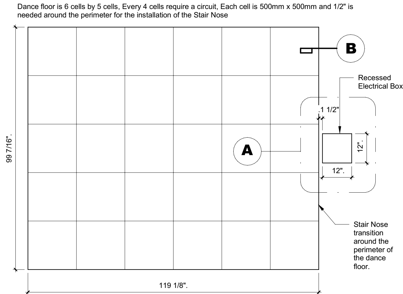
4 Dance Floor Recessed 1 1/2" = 1'-0"
