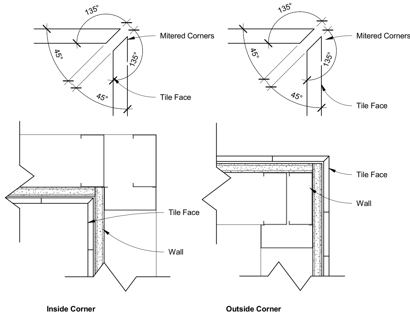
5 Typical Ceramic Tile Corner Detail N.T.S.
