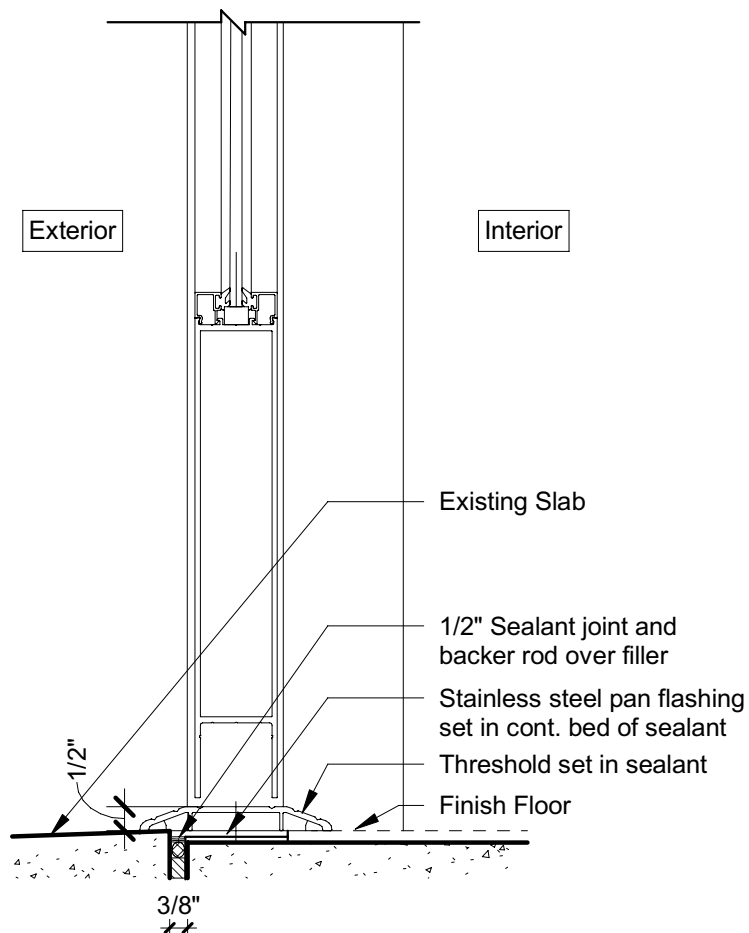
2 Storefront Sill detail 3" = 1'-0"
