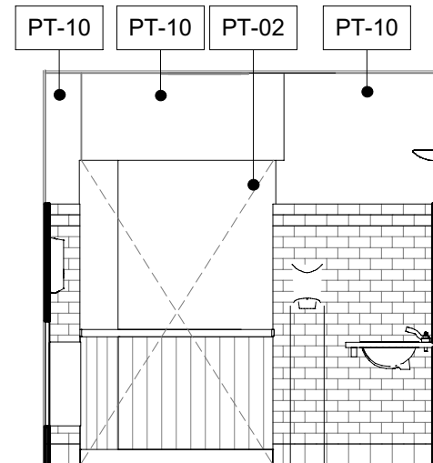
1/4'' = 1'-0''
