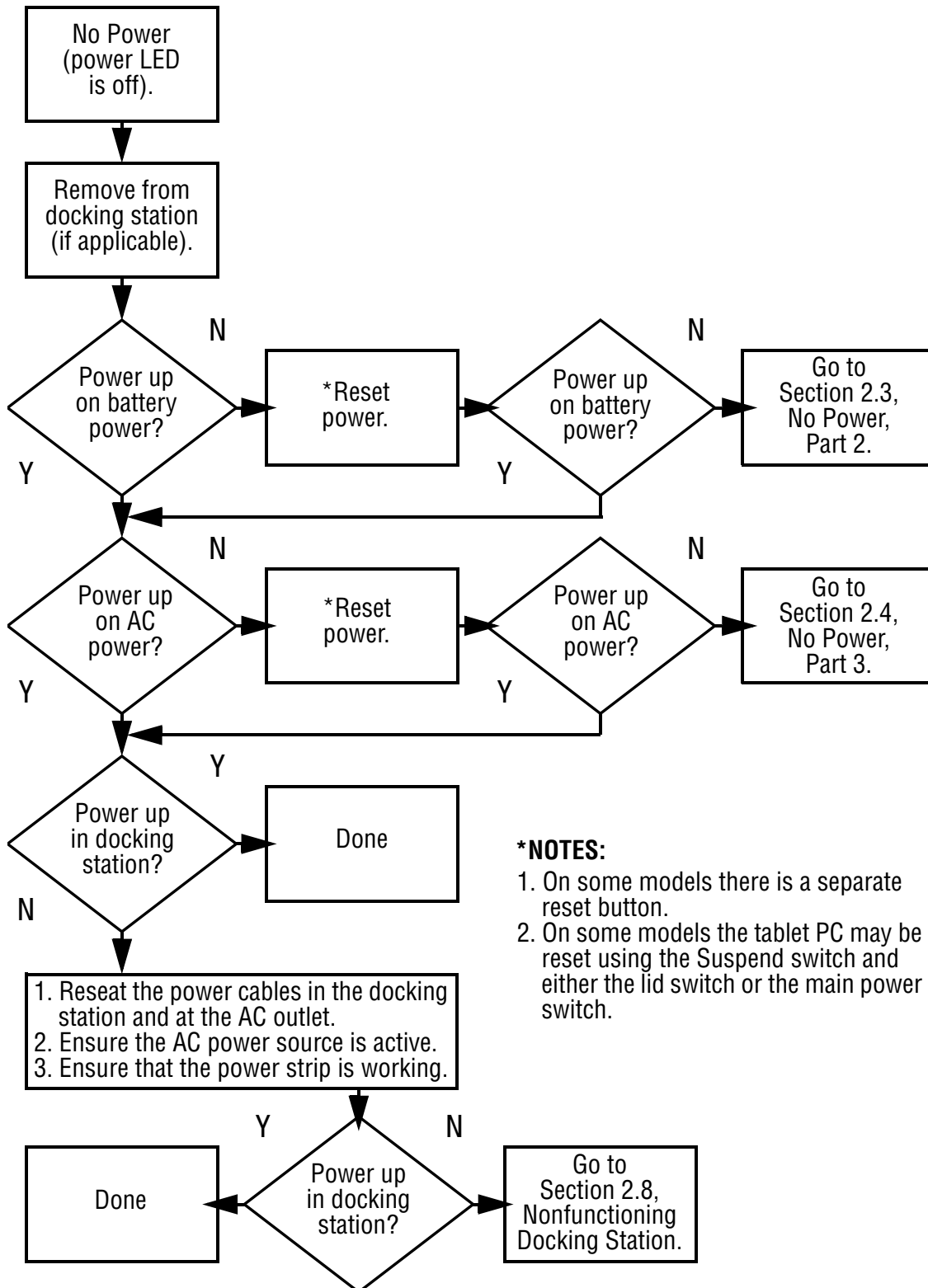
Flowchart 2.2—No Power, Part 1
