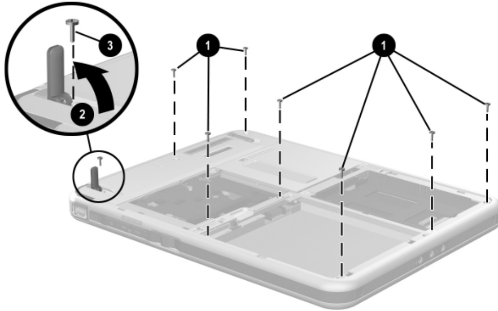
Figure 5-9. Removing the Display Panel Assembly Screws
