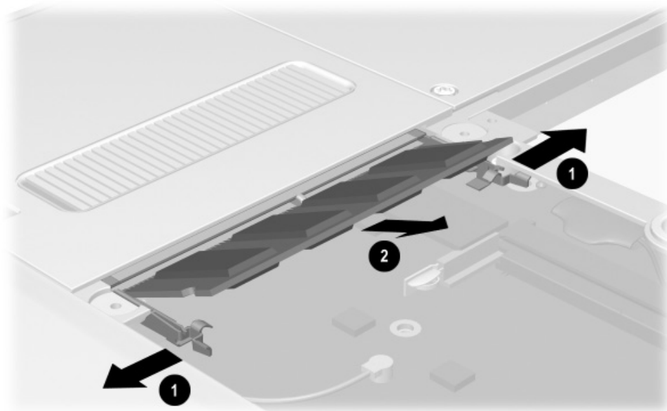
Figure 5-5. Removing the Memory Expansion Board
