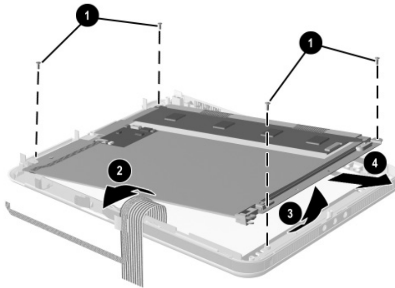
Figure 5-14. Removing the Display Panel
