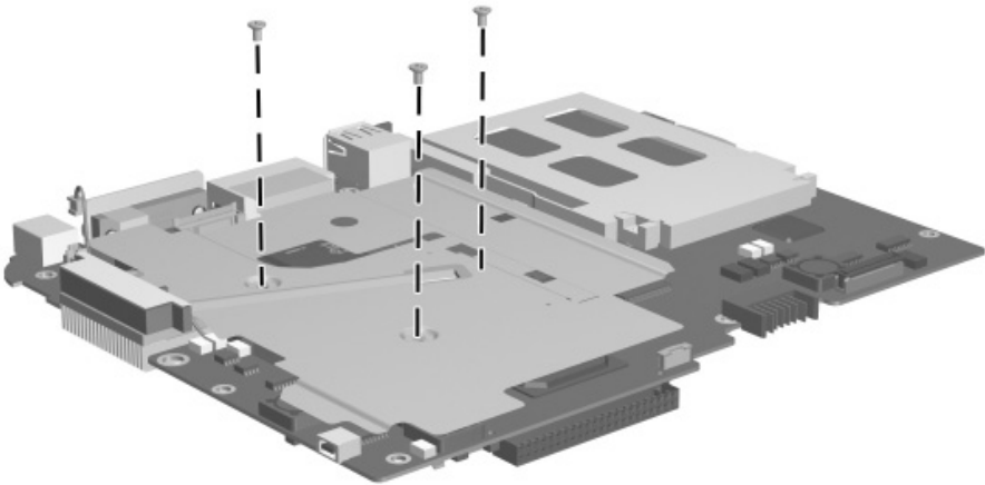
Figure C-9. Phillips M2.0 × 3.5 Screw Locations
