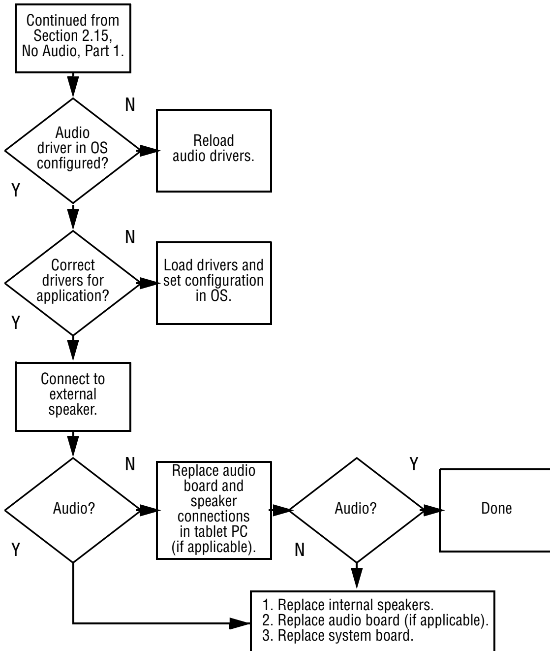
Flowchart 2.16—No Audio, Part 2
