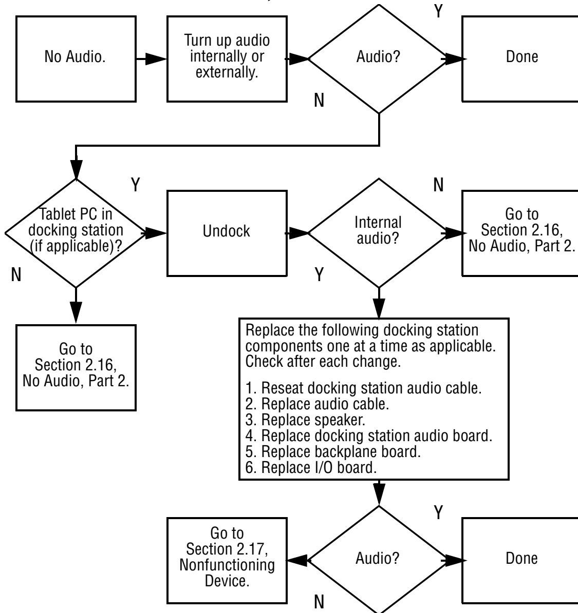
Flowchart 2.15—No Audio, Part 1
