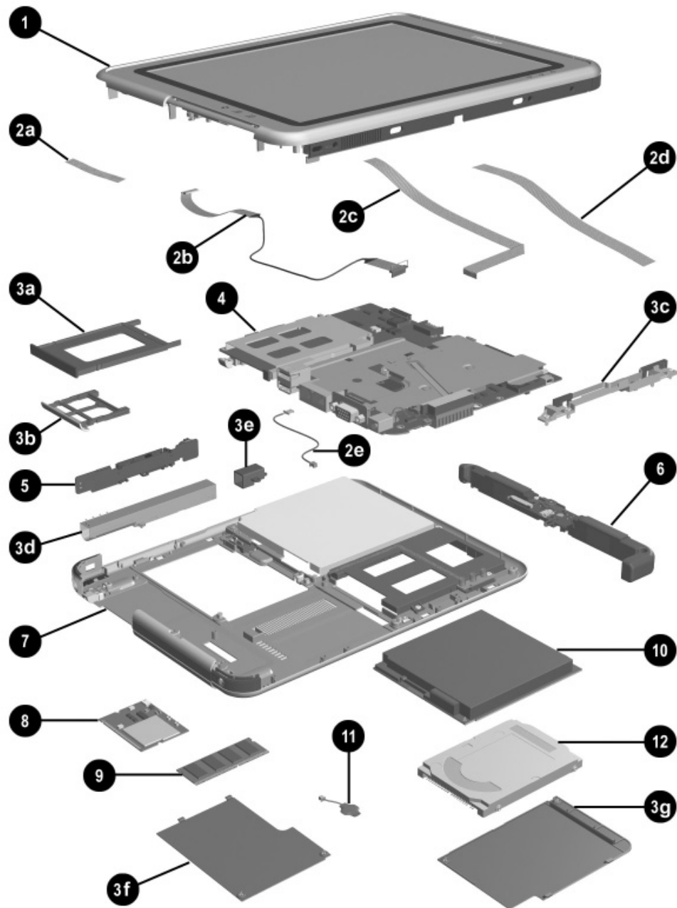
Figure 3-2. Tablet PC Major Components
