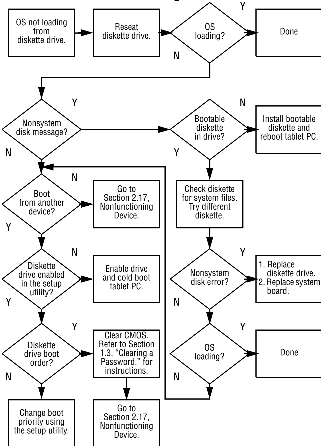
Flowchart 2.13—No OS Loading from Diskette Drive
