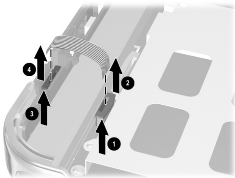
Figure 5-23. Removing the Switch Board Cable
