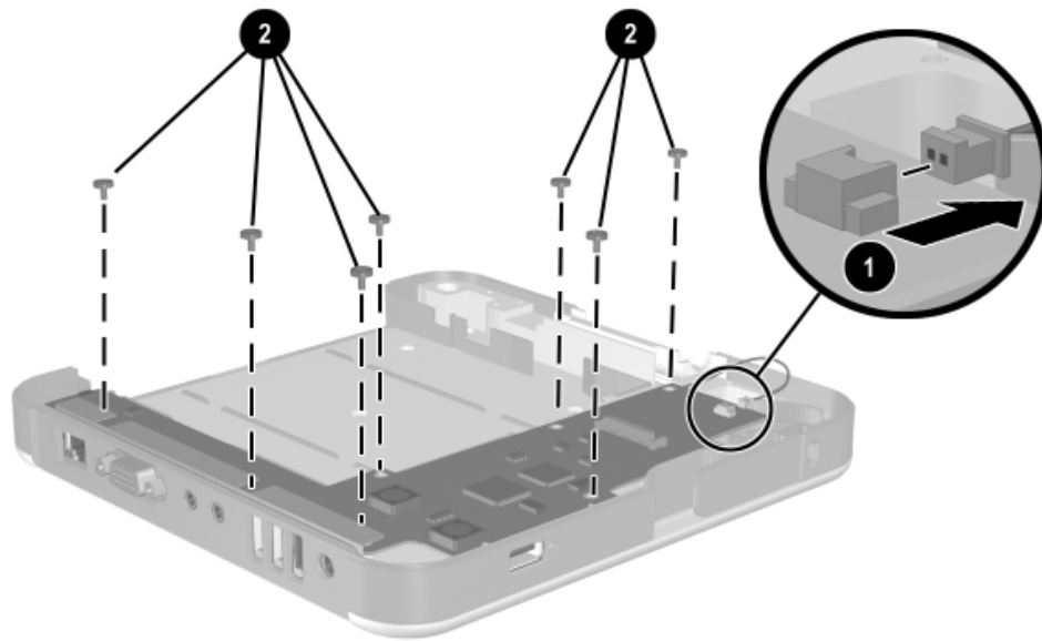
Figure 5-34. Removing the Board Assembly Screws
