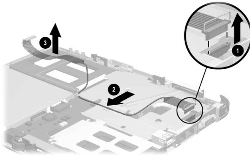
Figure 5-19. Removing the Digitizer Cable
