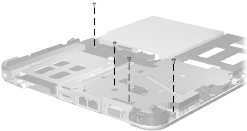
Figure C-7. Phillips M2.0 × 5.0 Screw Locations
