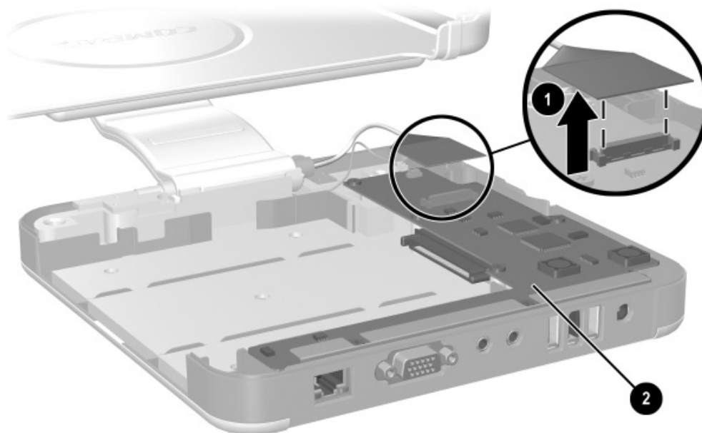
Figure 5-32. Disconnecting the Docking Stand Cable
