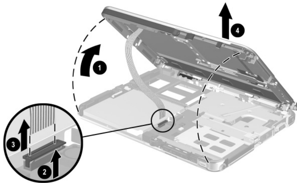
Figure 5-11. Removing the Display Panel Assembly
