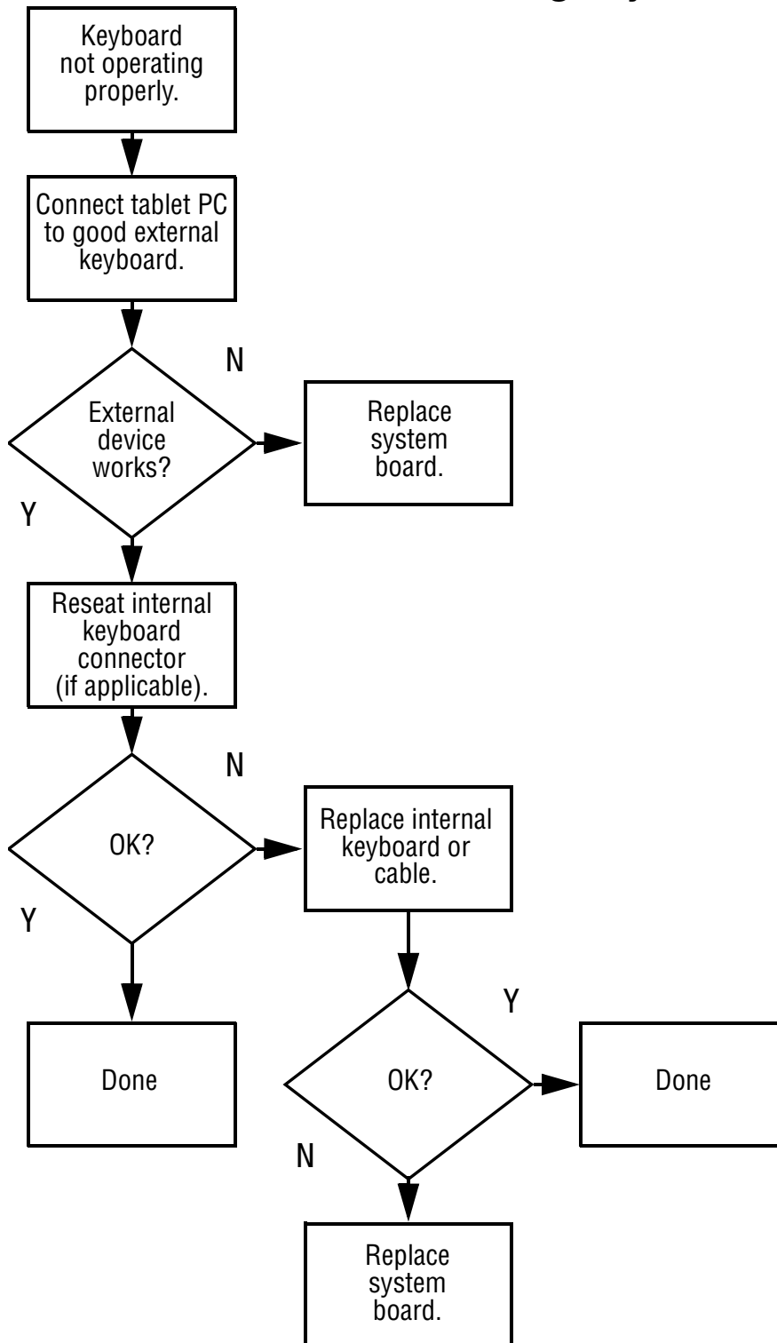
Flowchart 2.18—Nonfunctioning Keyboard
