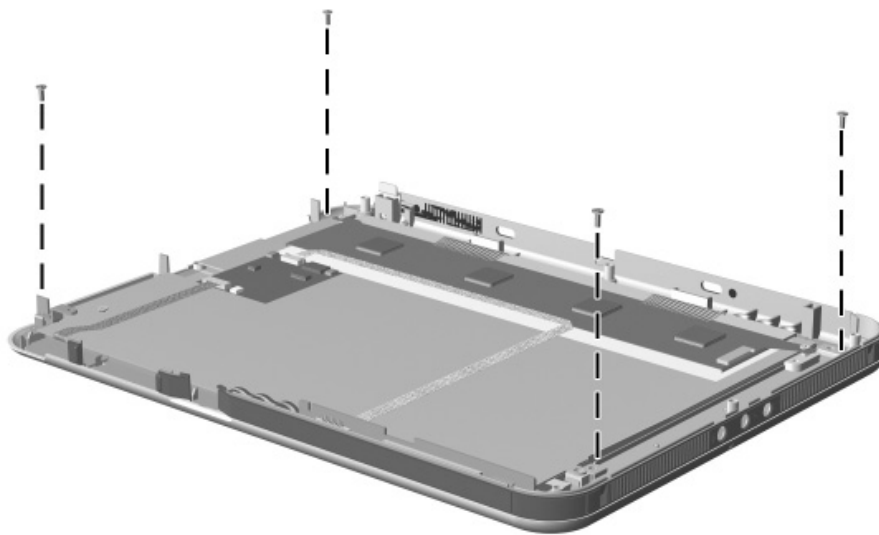
Figure C-2. Phillips M2.0 × 4.0 Screw Locations
