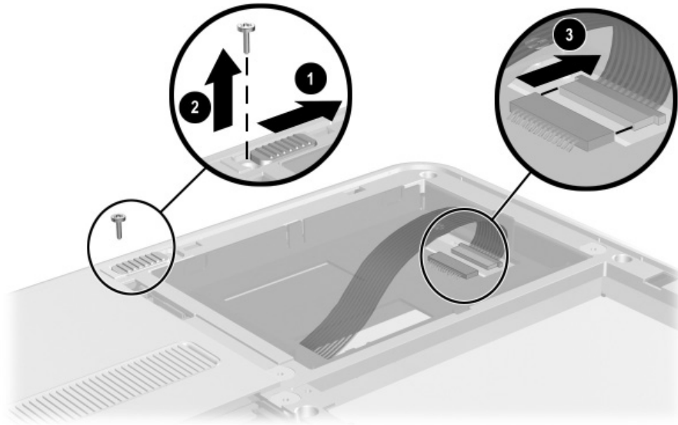
Figure 5-10. Removing the Display Panel Assembly Screw and Disconnecting the Digitizer Cable
