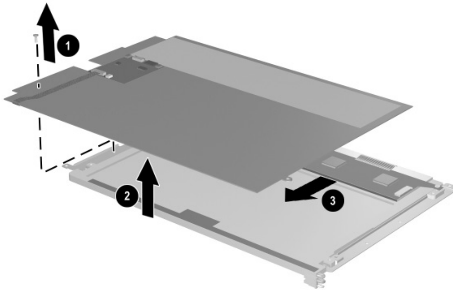
Figure 5-15. Removing the Digitizer
