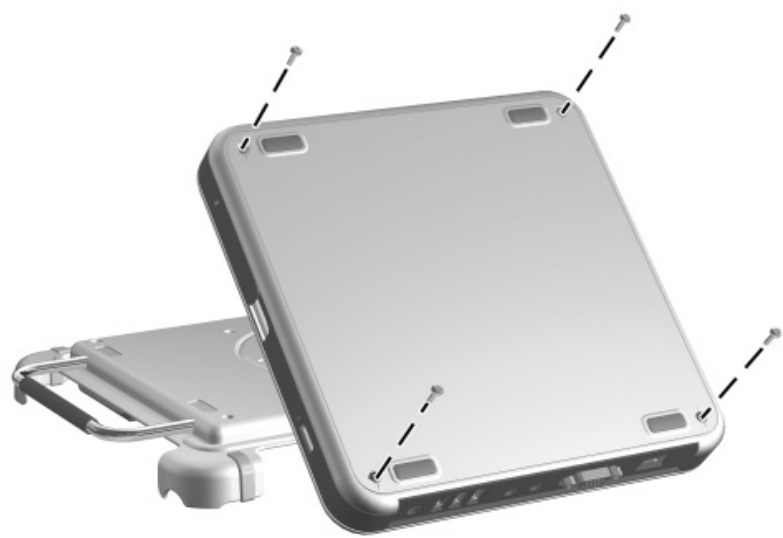
Figure C-5. Torx M2.5 × 7.0 Screw Locations
