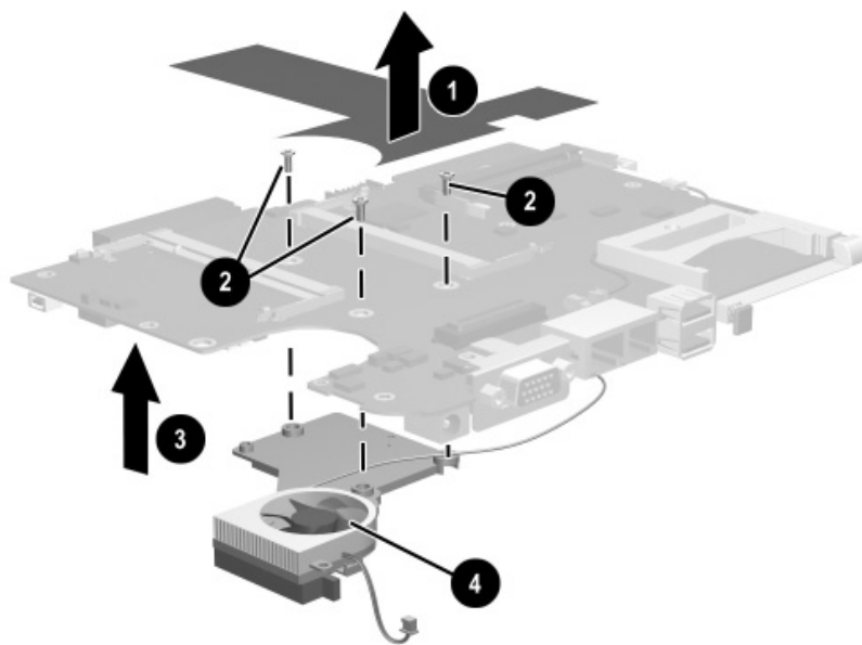
Figure 5-27. Removing the Fan and Heat Sink
