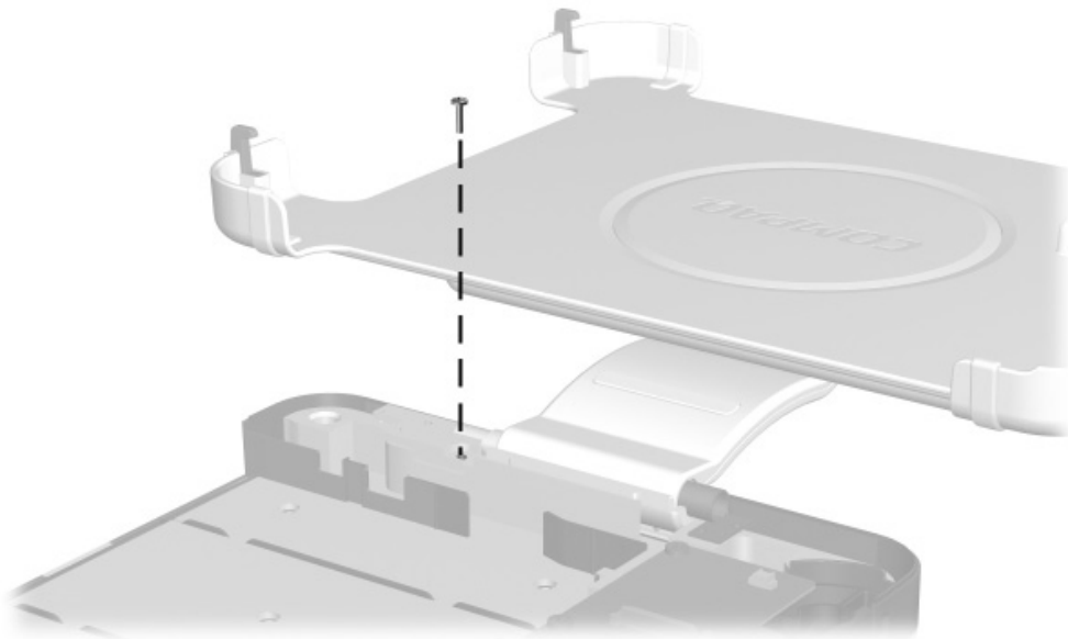
Figure C-12. Phillips M2.5 × 12.0 Screw Location
