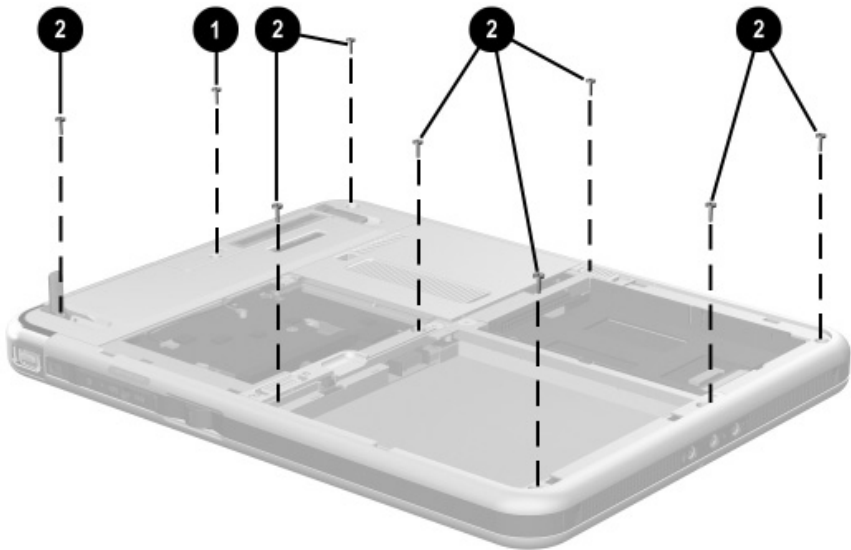
Figure C-3. Torx M2.5 × 7.0 Screw Locations
