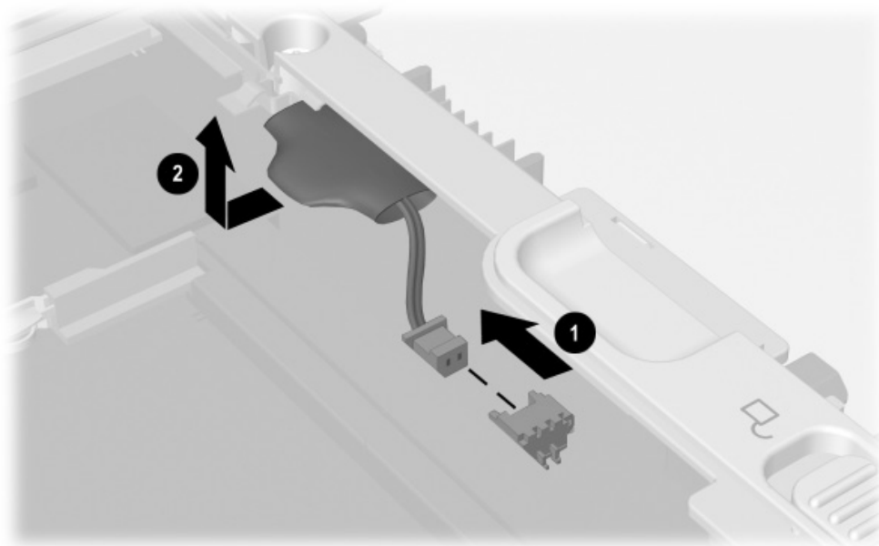
Figure 5-8. Removing the RTC Battery
