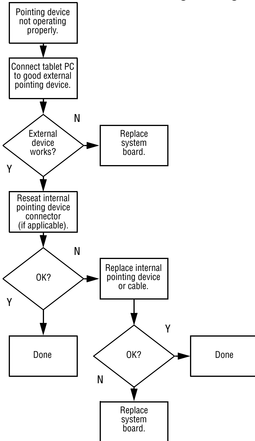
Flowchart 2.19—Nonfunctioning Pointing Device
