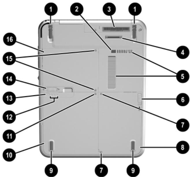
Figure 1-8. Bottom Components
