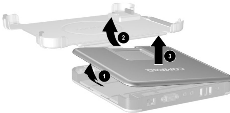
Figure 5-31. Removing the Top Case
