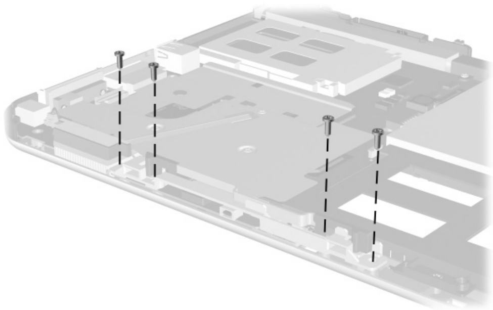
Figure C-4. Torx M2.5 × 7.0 Screw Locations
