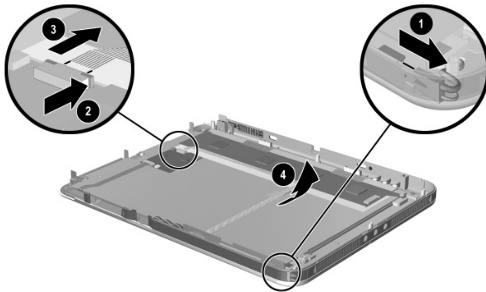
Figure 5-13. Disconnecting the Display Panel Cables
