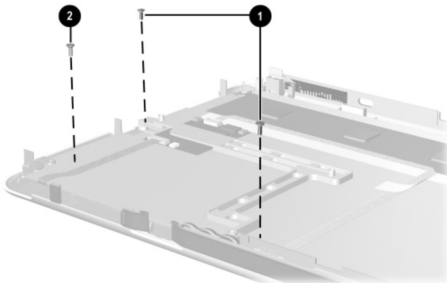
Figure C-6. Phillips M2.0 × 5.0 Screw Locations
