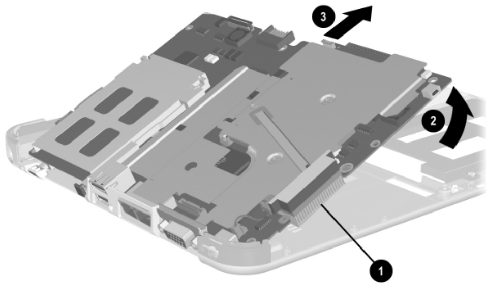
Figure 5-25. Removing the System Board
