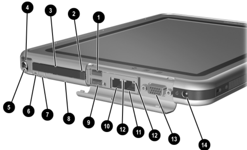
Figure 1-4. Top Side Components
