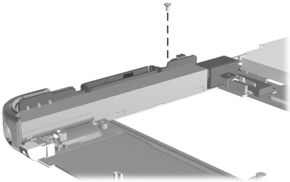
Figure C-10. Phillips M2.0 × 3.5 Screw Locations
