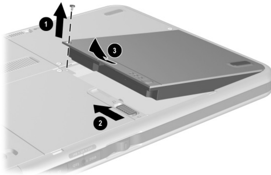
Figure 5-2. Removing the Battery Pack
