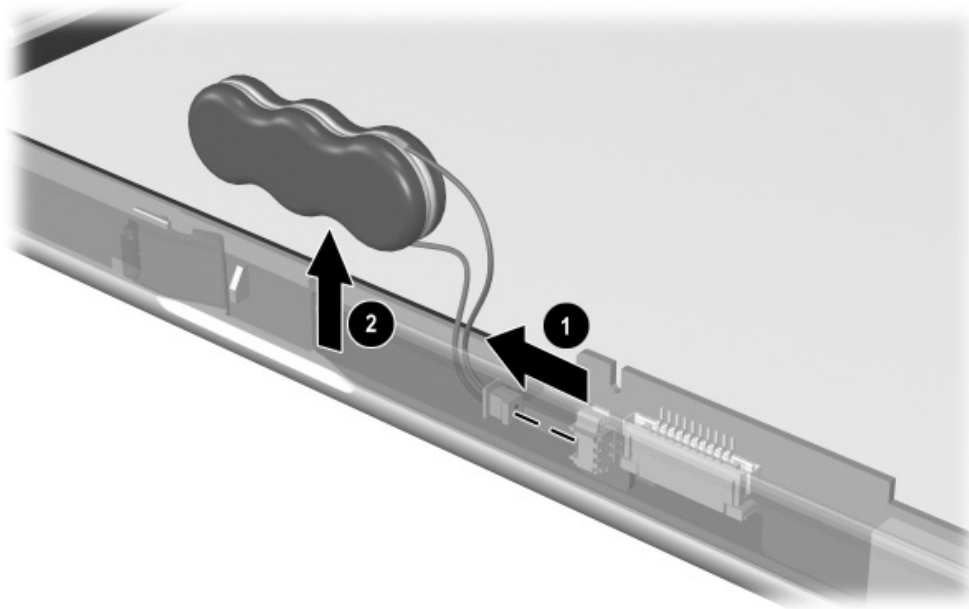
Figure 5-16. Removing the Bridge Battery
