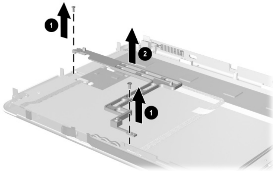
Figure 5-12. Removing the Display Panel Bracket
