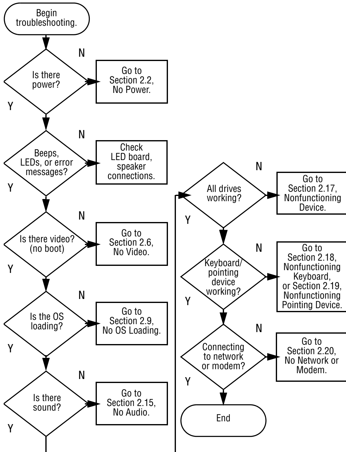
Flowchart 2.1—Initial Troubleshooting
