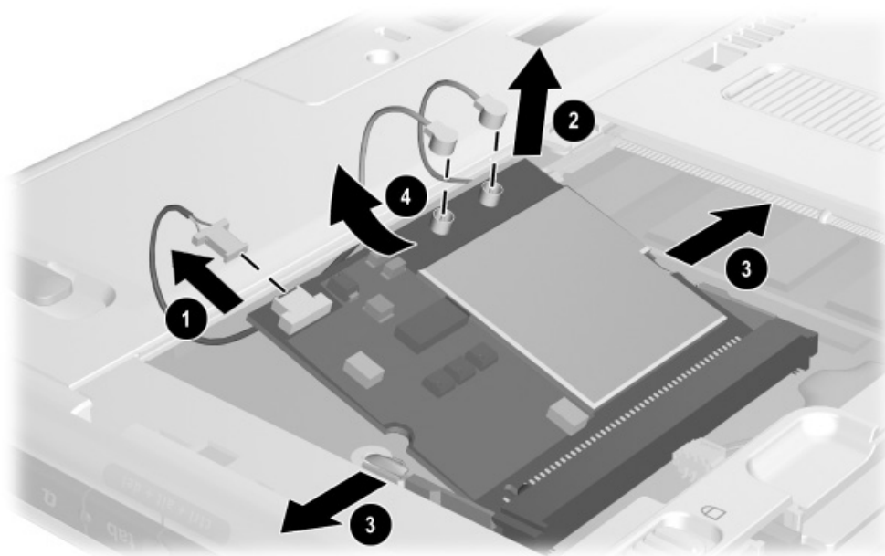
Figure 5-4. Removing the Mini PCI Communications Board
