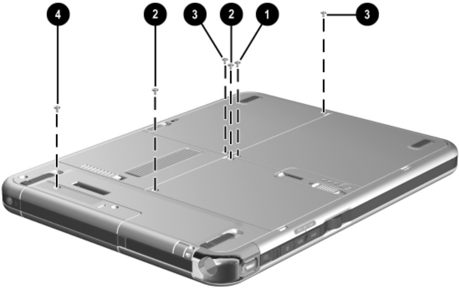
Figure C-1. Phillips M2.0 × 4.0 Screw Location
