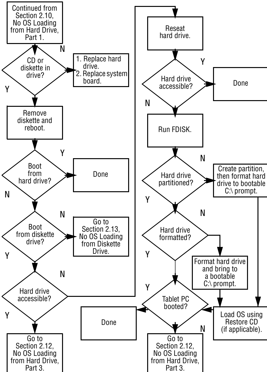
Flowchart 2.11—No OS Loading from Hard Drive, Part 2
