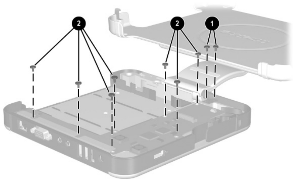
Figure C-11. Phillips M2.5 × 5.0 Screw Locations
