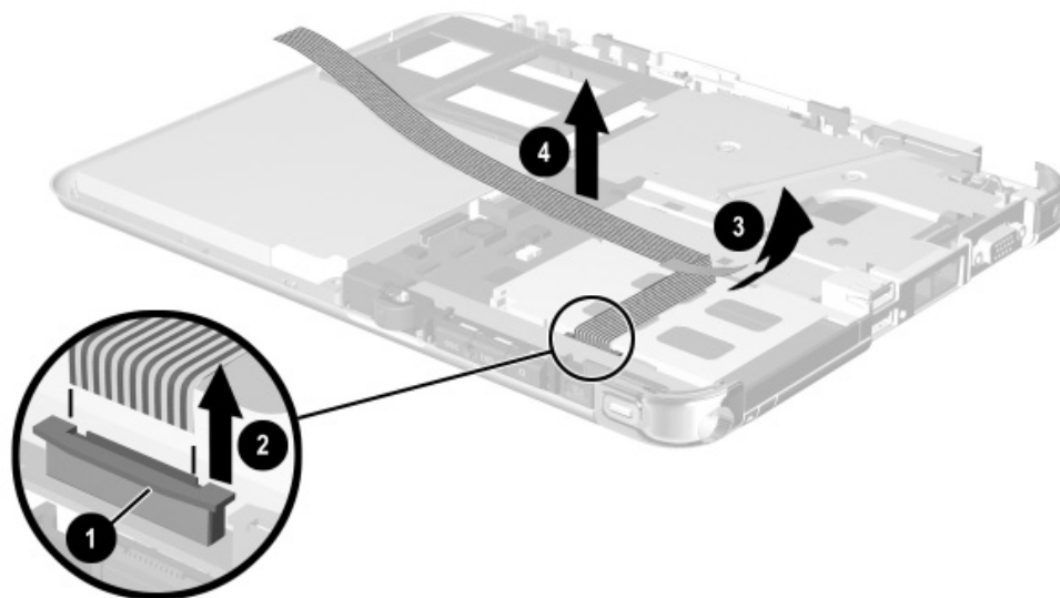
Figure 5-18. Removing the Speaker Cable
