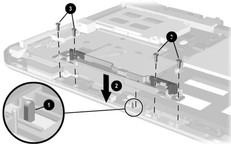
Figure 5-21. Installing the Keyboard Release Assembly
