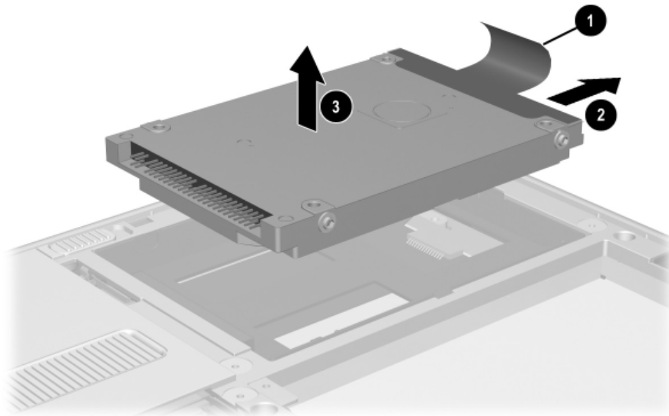
Figure 5-7. Removing the Hard Drive
