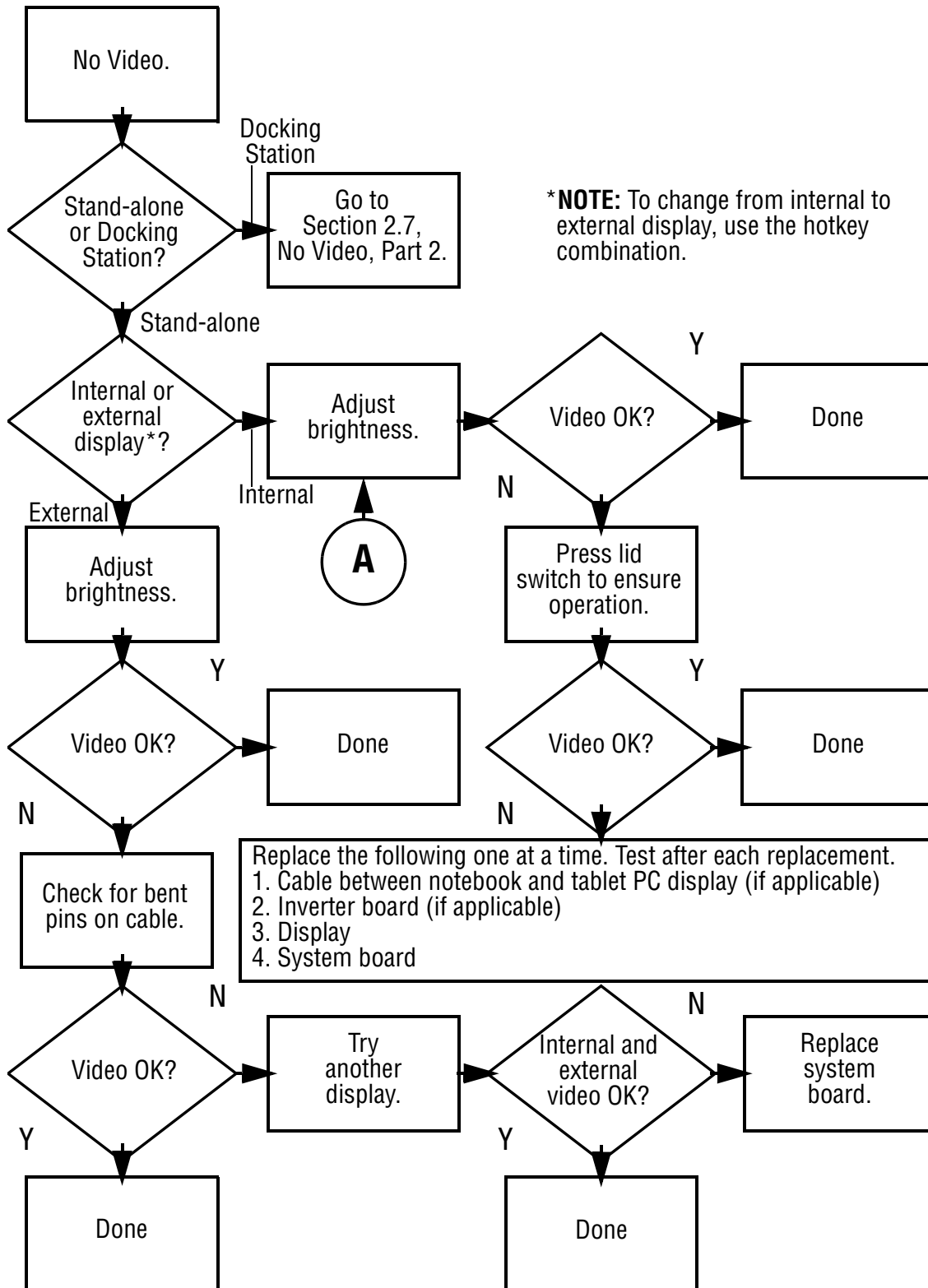
Flowchart 2.6—No Video, Part 1
