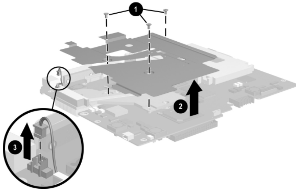
Figure 5-26. Removing the EMI Shield
