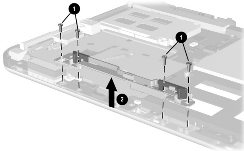
Figure 5-20. Removing the Keyboard Release Assembly
