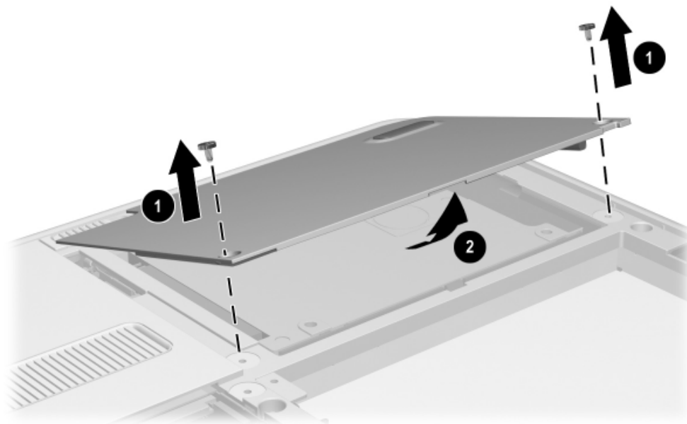
Figure 5-6. Removing the Hard Drive Cover
