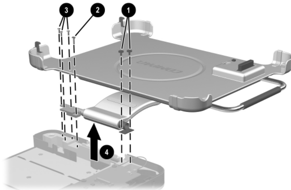
Figure 5-33. Removing the Docking Stand and Pivot Arm
