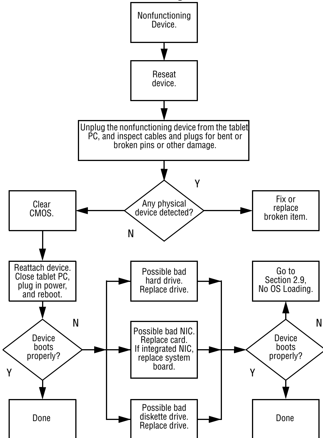
Flowchart 2.17—Nonfunctioning Device
