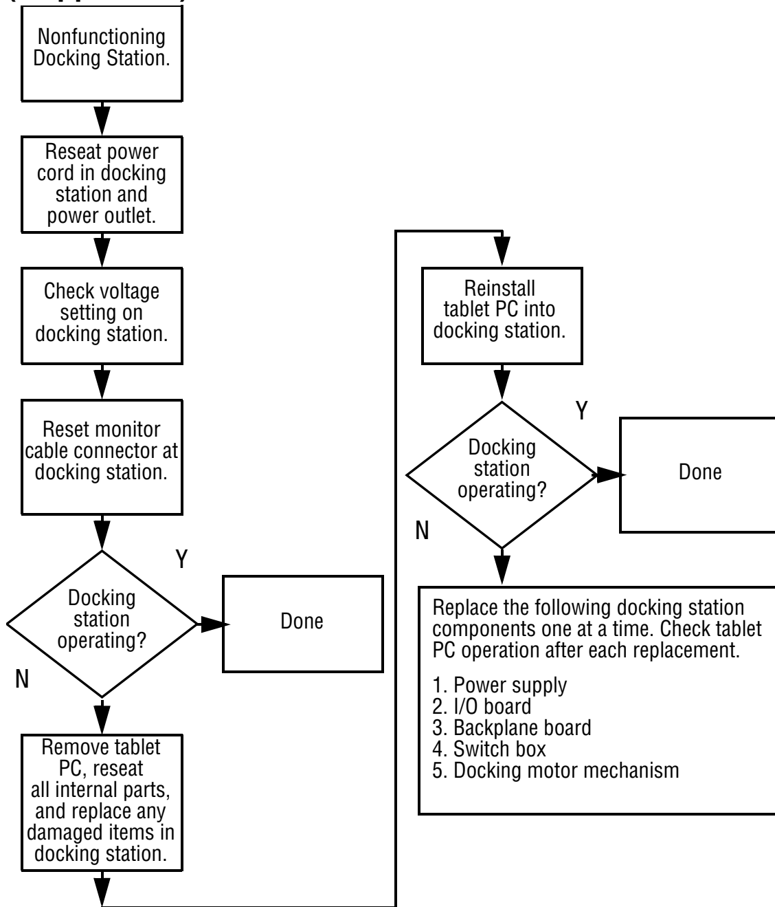
Flowchart 2.8—Nonfunctioning Docking Station (if applicable)
