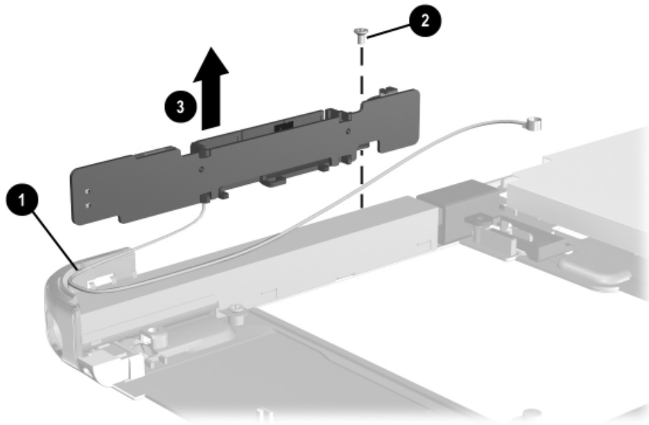
Figure 5-29. Removing the Switch Board
