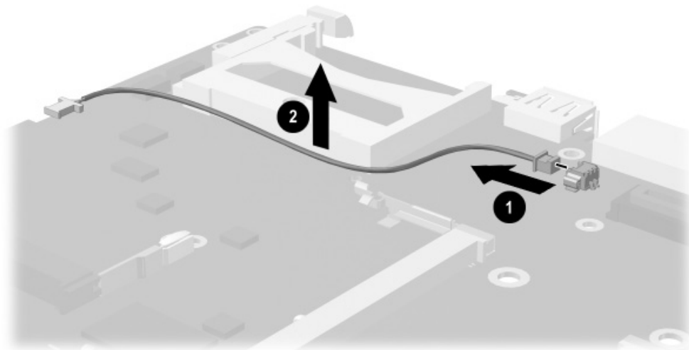
Figure 5-28. Removing the Modem Cable
