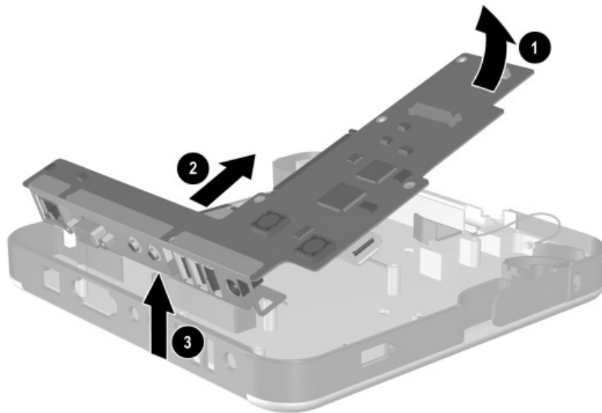
Figure 5-35. Removing the Board Assembly
