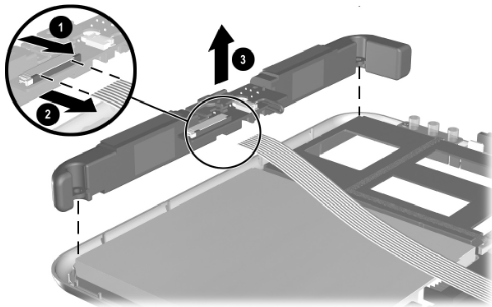
Figure 5-17. Removing the Speaker Assembly
