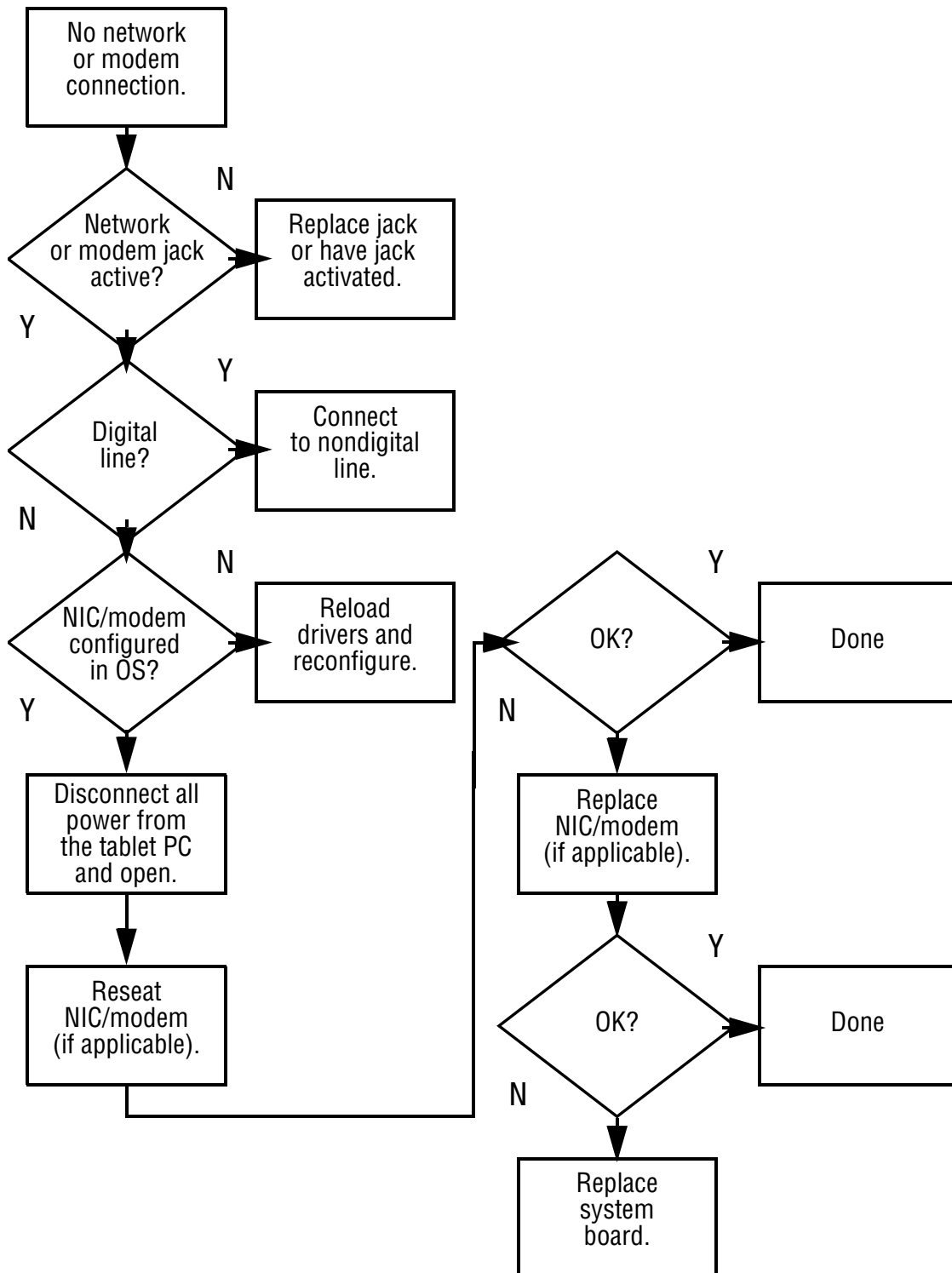
Flowchart 2.20—No Network or Modem Connection
